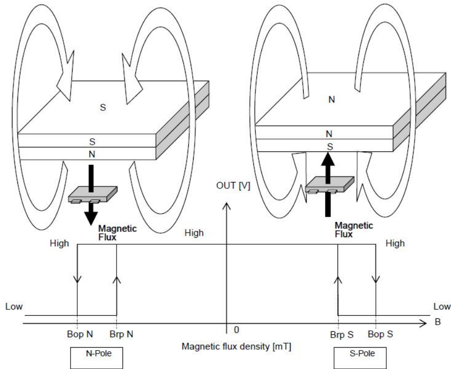
Fig 4, Magnetic Operation Characteristic of AS1895
