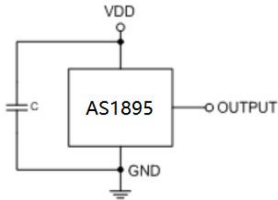
Figure 1, Typical Application Circuit of AS1895
