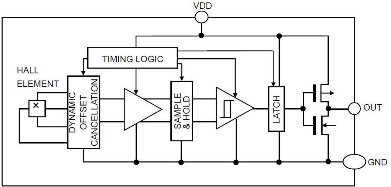
Figure 3, Block Diagram of AS1895
